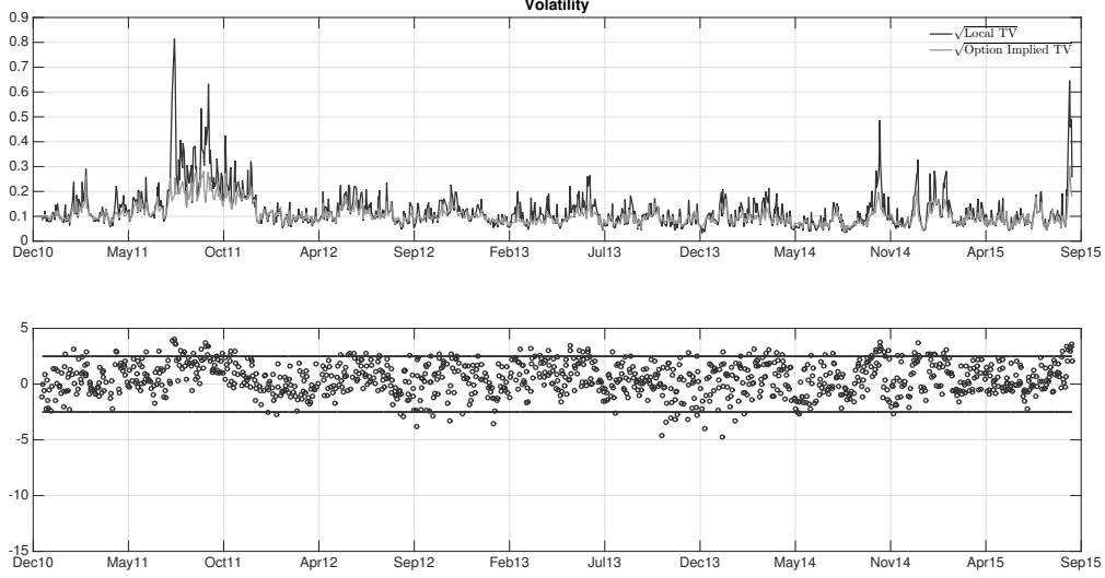
Figure 10: Volatility fit based on the semi-nonparametric model (12). The top panel reports end-of-day spot volatilities based on nonparametric estimates from high-frequency data (solid line) or option-implied values (grey line). The option-implied volatility estimate is based on the semi-nonparametric model (12) with \alpha = 0.5 and the state vector estimated from the short-maturity option sample. The volatility estimates are reported in annualized units. The bottom panel reports the corresponding daily volatility test statistics (8). The solid lines indicate the symmetric 95% confidence band for the test.
