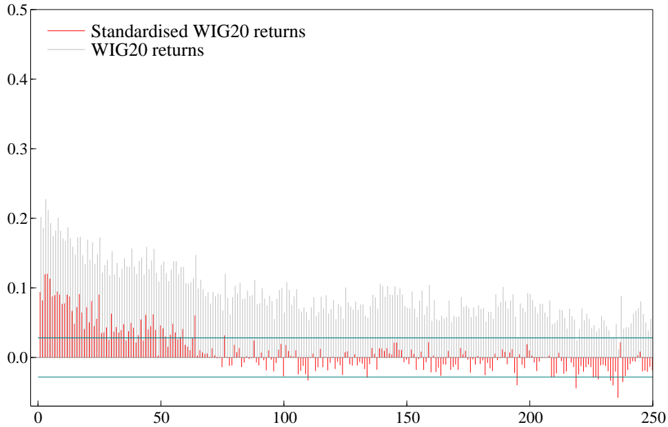
Figure 3: First 250 autocorrelations of absolute values |\varepsilon_t| of the WIG20 index and the rescaled series |\varepsilon_t|/\widehat{g}_t^{1/2} .
