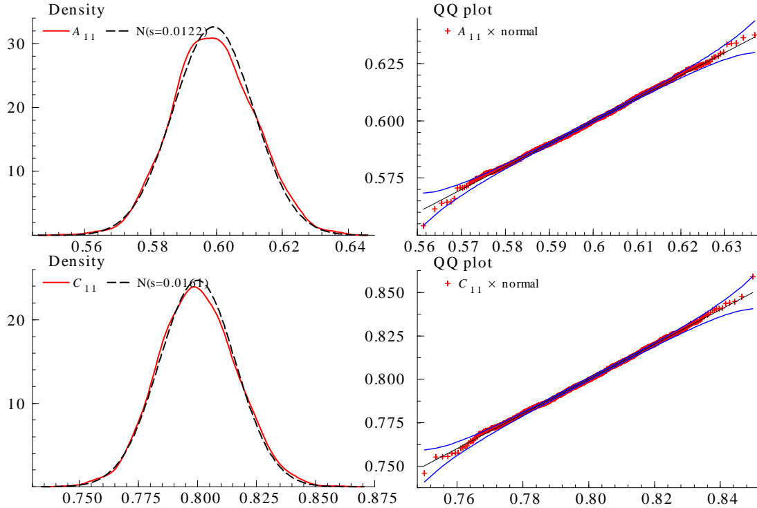
Figure 5.1: Density and Q-Q plots of N = 1000 VT estimates of A_{11} and C_{11} of the process (5.1)-(5.3). In the density plots the red line is the plot of the estimated density of the VT estimates, and the black dashed line is the plot for the normal distribution. The Q-Q plots compare the quantiles of the estimate with the ones of a normal distribution (red crosses). The solid blue lines are the asymptotic 95% standard error bands of a normal distribution.
