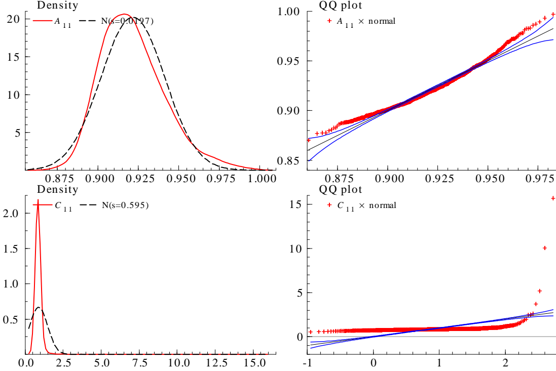
Figure 5.3: Density and Q-Q plots of N = 1000 VT estimates of A_{11} and C_{11} of the process (5.1),(5.2),(5.6). In the density plots the red line is the plot of the estimated density of the VT estimates, and the black dashed line is the plot for the normal distribution. The Q-Q plots compare the quantiles of the estimate with the ones of a normal distribution (red crosses). The solid blue lines are the asymptotic 95% standard error bands of a normal distribution.
