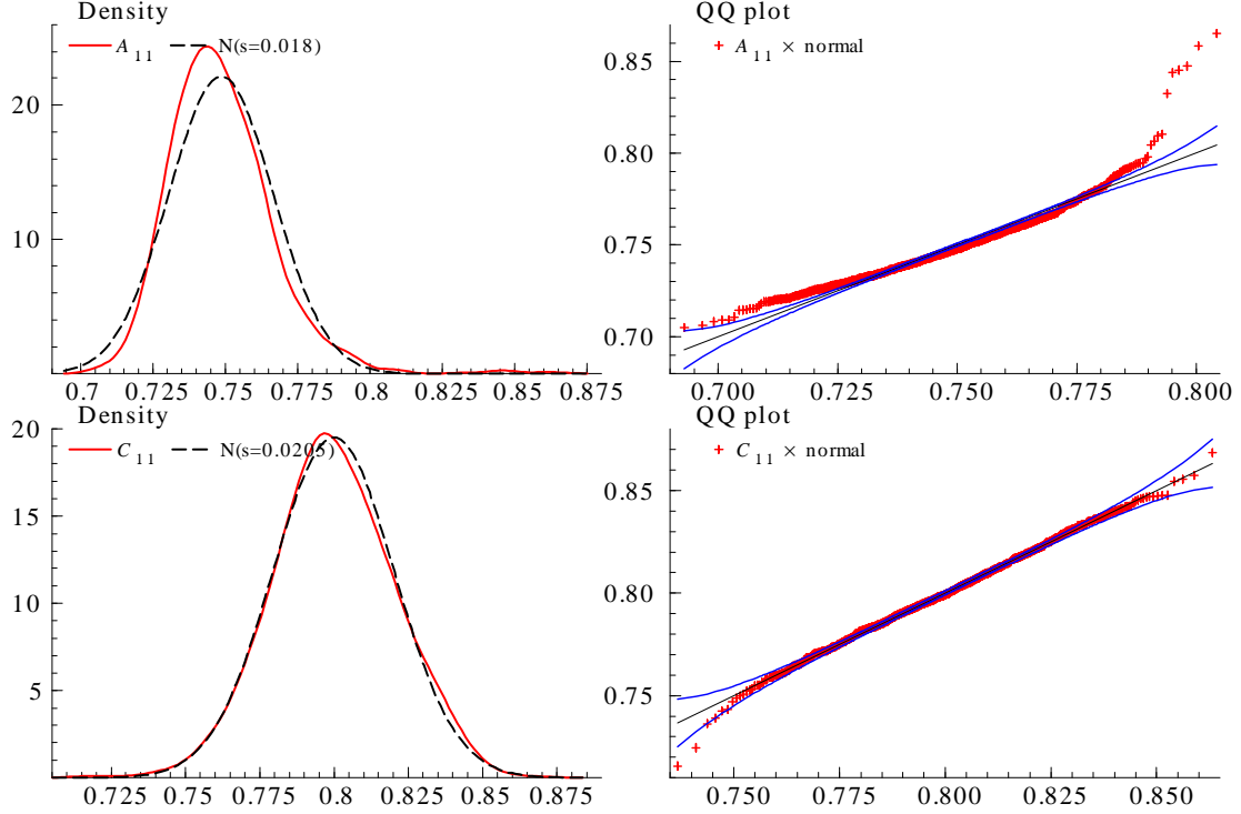
Figure 5.2: Density and Q-Q plots of N = 1000 VT estimates of A_{11} and C_{11} of the process (5.1),(5.2),(5.4). In the density plots the red line is the plot of the estimated density of the VT estimates, and the black dashed line is the plot for the normal distribution. The Q-Q plots compare the quantiles of the estimate with the ones of a normal distribution (red crosses). The solid blue lines are the asymptotic 95% standard error bands of a normal distribution.
