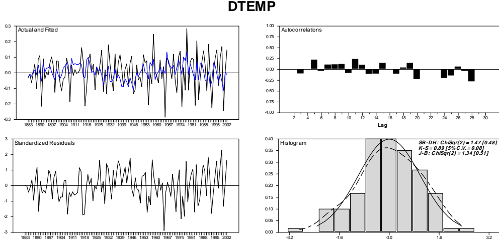
Figure 6: Plot of actual and fitted values of \Delta T_t , the normalized residuals, their autocorrelation function and histogram.
