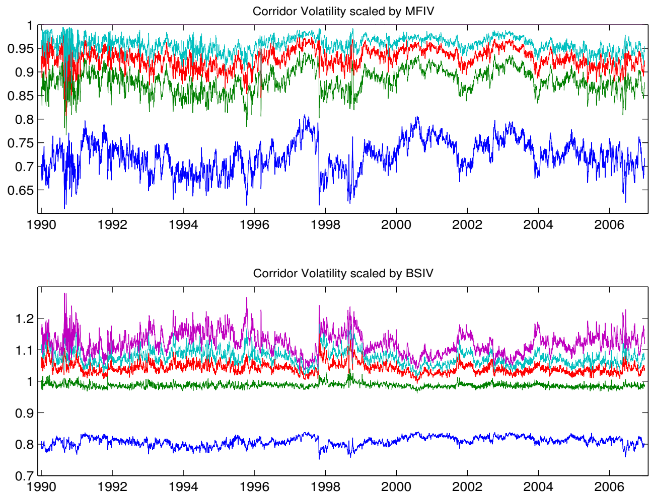
Figure 4: The top panel plots the corridor variances CIV1-CIV4 scaled by MFIV. The bottom panel plots the corridor variances CIV1-CIV4 and MFIV scaled by BSIV.
